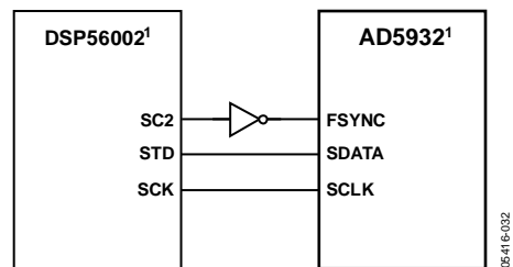
1 ADDITIONAL PINS OMITTED FOR CLARITY. Figure 37. DSP56002 to AD5932 Interface
