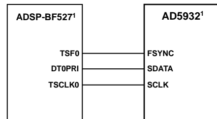
Figure 34. ADSP-BF527 to AD5932 Interface
