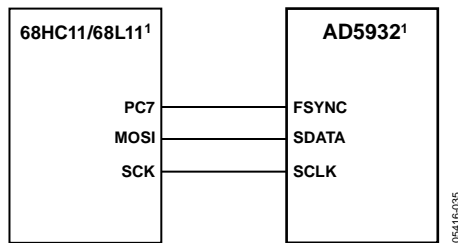
1 ADDITIONAL PINS OMITTED FOR CLARITY. Figure 35. 68HC11/68L11 to AD5932 Interface
