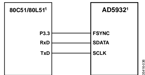
1 ADDITIONAL PINS OMITTED FOR CLARITY. Figure 36. 80C51/80L51 to AD5932 Interface
