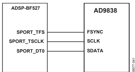
Figure 31. SDP to AD9838 Interface
