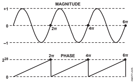
Figure 20. Sine Wave
